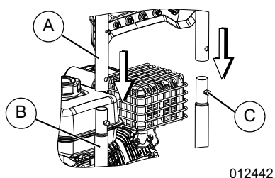
Figure 2-1. Enfiler le guidon
